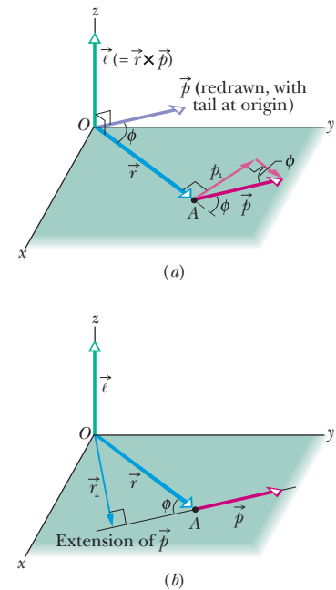
Figure 11-12 Defining angular momentum. A particle passing through point A has linear momentum \vec{p} (= m\vec{v}) , with the vector \vec{p} lying in an xy plane. The particle has angular momentum \vec{\ell} (= \vec{r} \times \vec{p}) with respect to the origin O . By the right-hand rule, the angular momentum vector points in the positive direction of z . (a) The magnitude of \vec{\ell} is given by \ell = rp_{\perp} = rmv_{\perp} . (b) The magnitude of \vec{\ell} is also given by \ell = r_{\perp} p = r_{\perp} mv .
