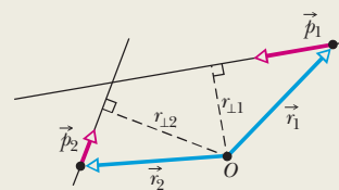
Figure 11-13 Two particles pass near point O .
